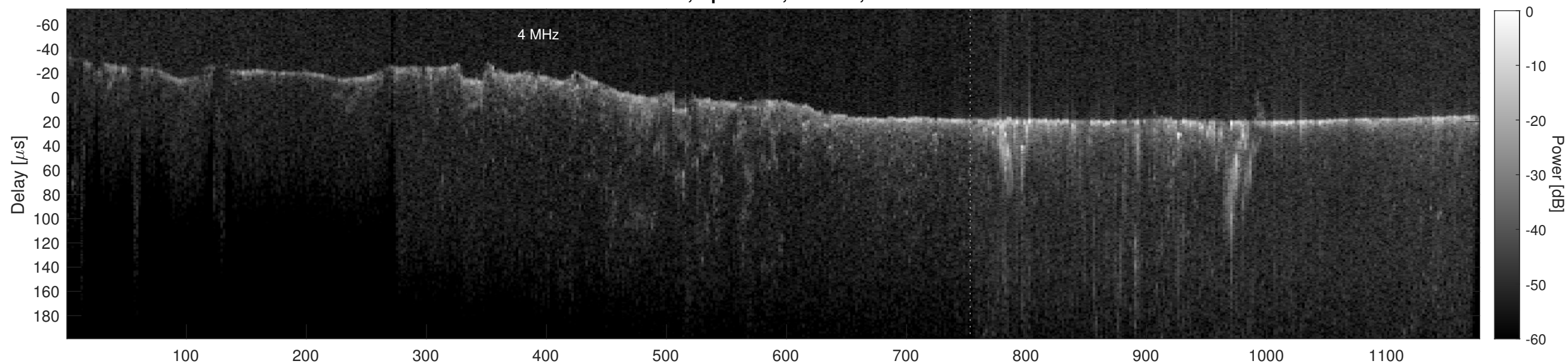
Orbit 18724, Cluttergram
