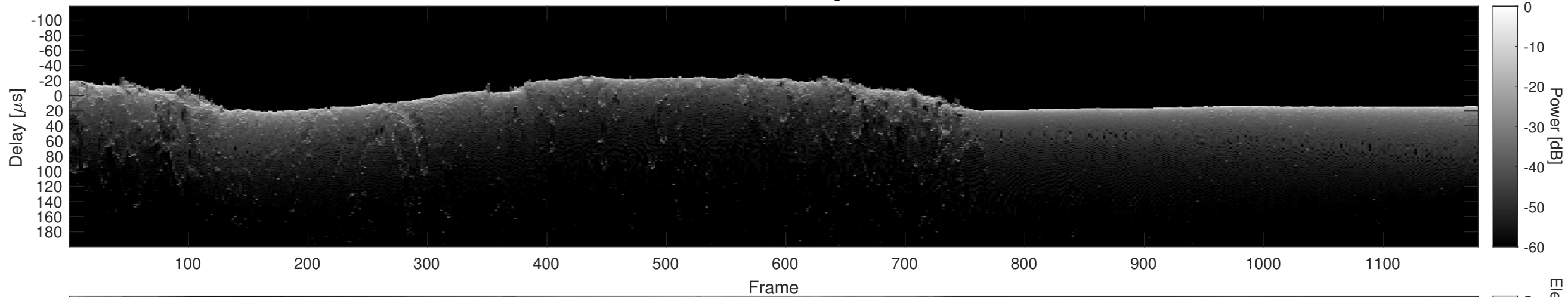
Orbit 18725, Cluttergram
