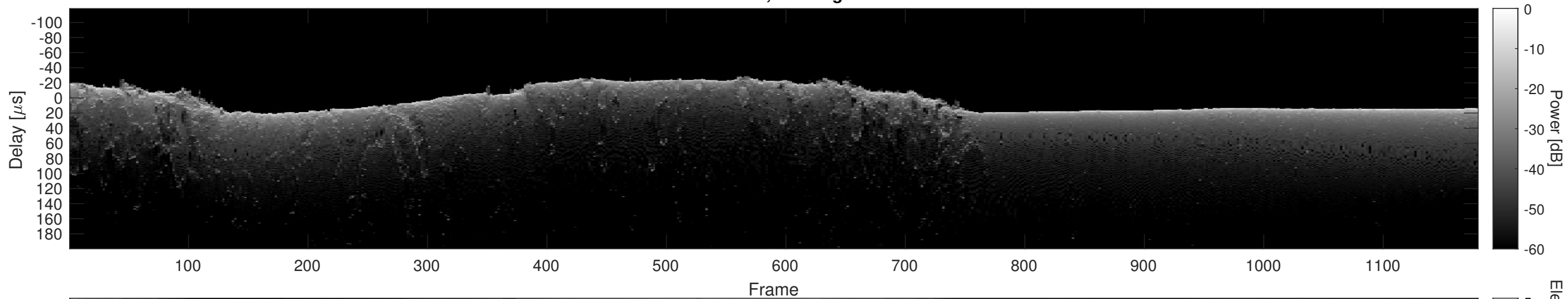
Orbit 18725, Cluttergram
