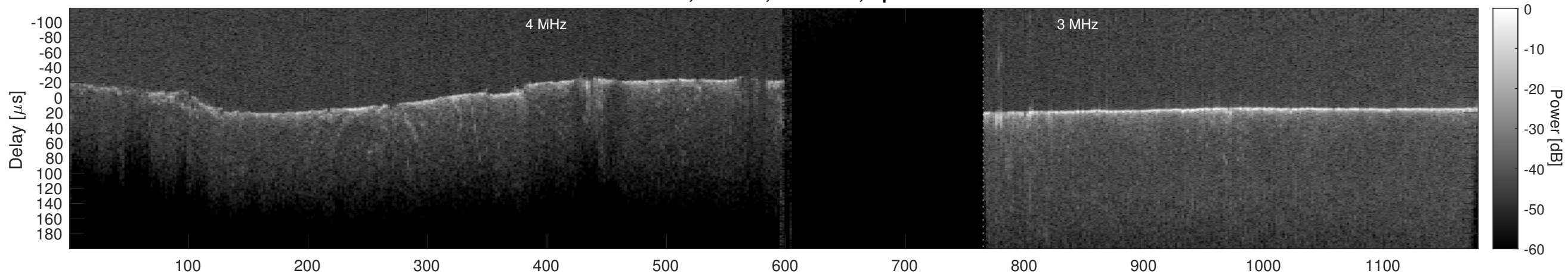
Orbit 18725, Cluttergram
