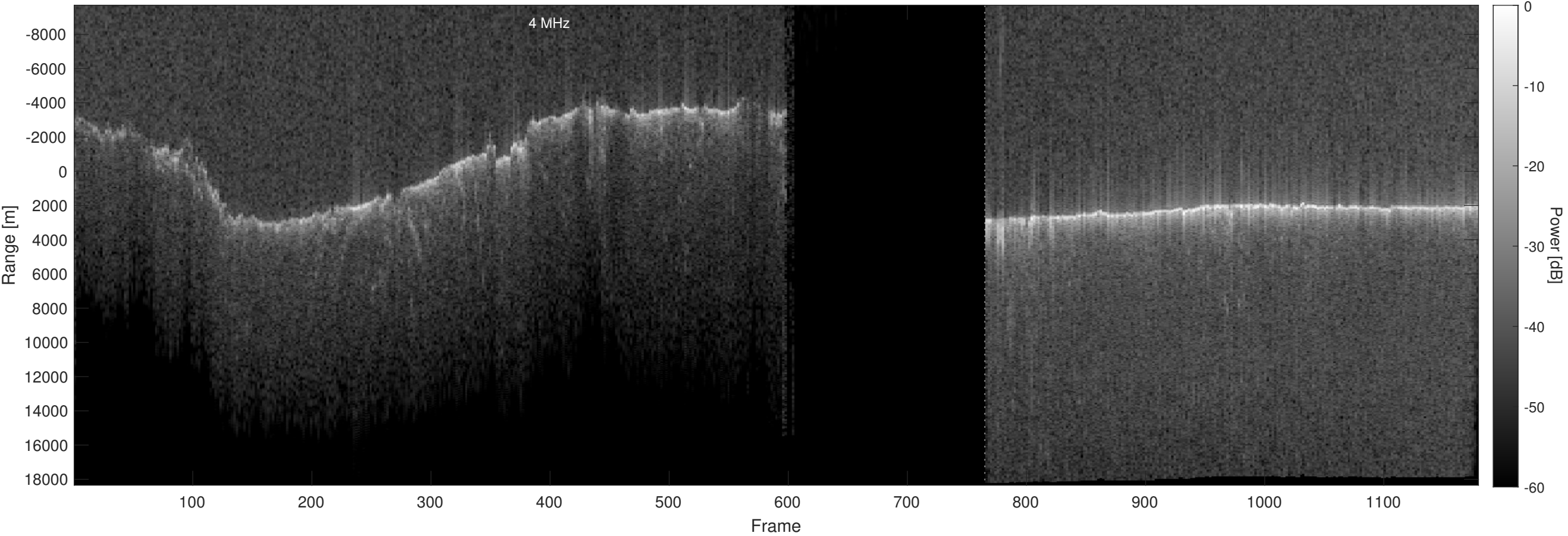
Orbit 18725, Optimized, No Window, Depth-Corrected, Channel 2
