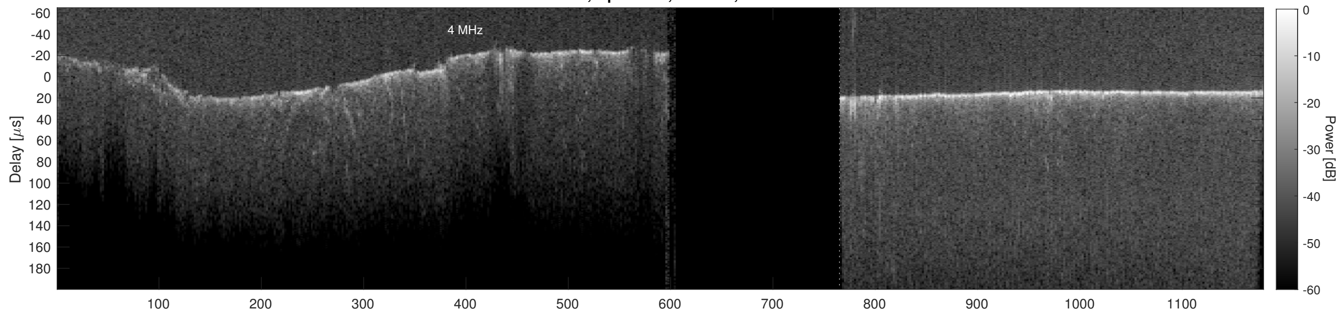
Orbit 18725, Cluttergram
