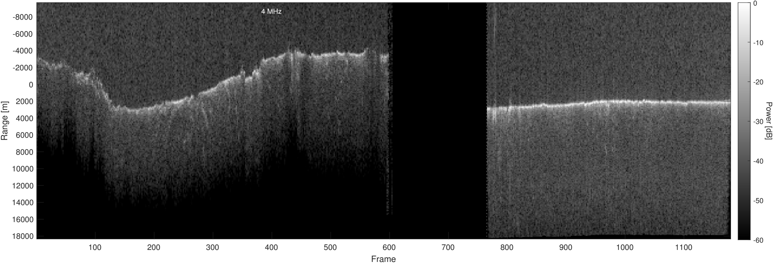
Orbit 18725, Optimized, Window, Depth-Corrected, Channel 2
