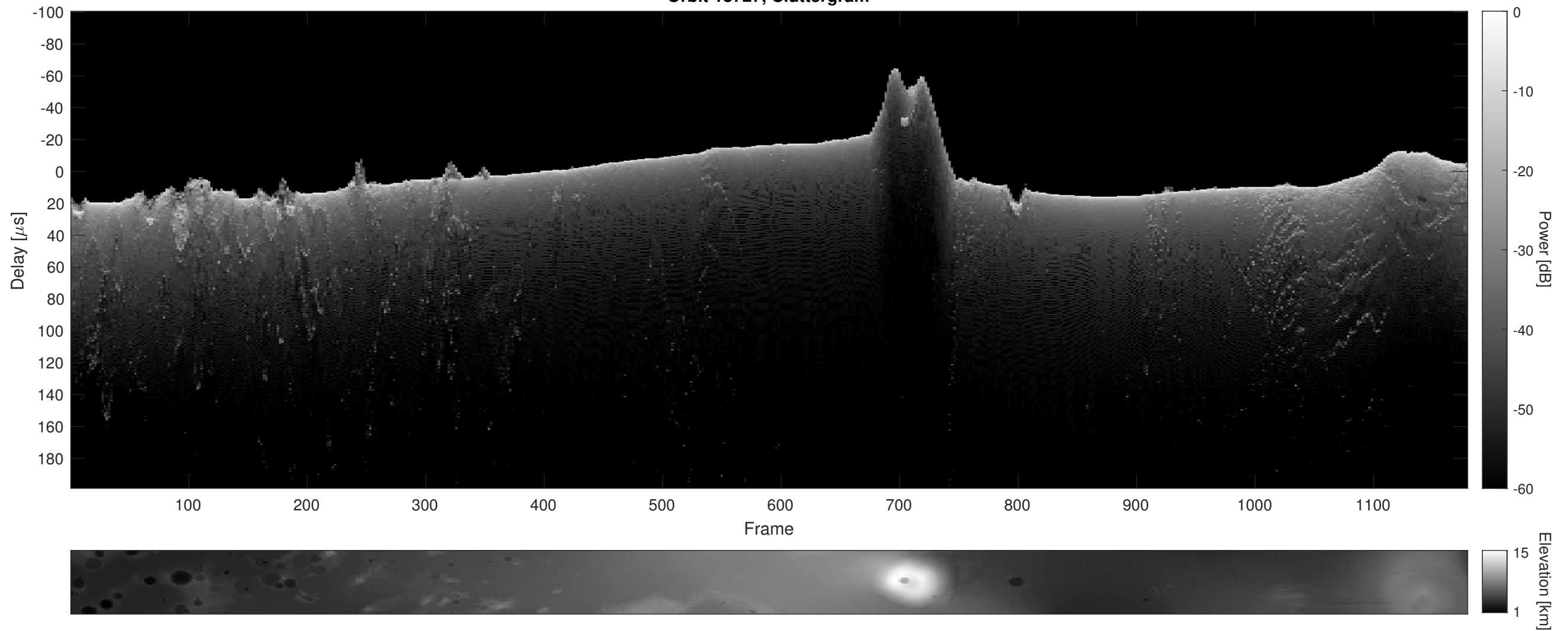
Orbit 18727, Cluttergram
