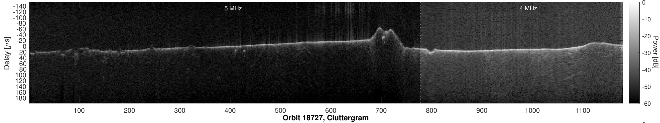
Orbit 18727, Window, Channel 1, Optimized
