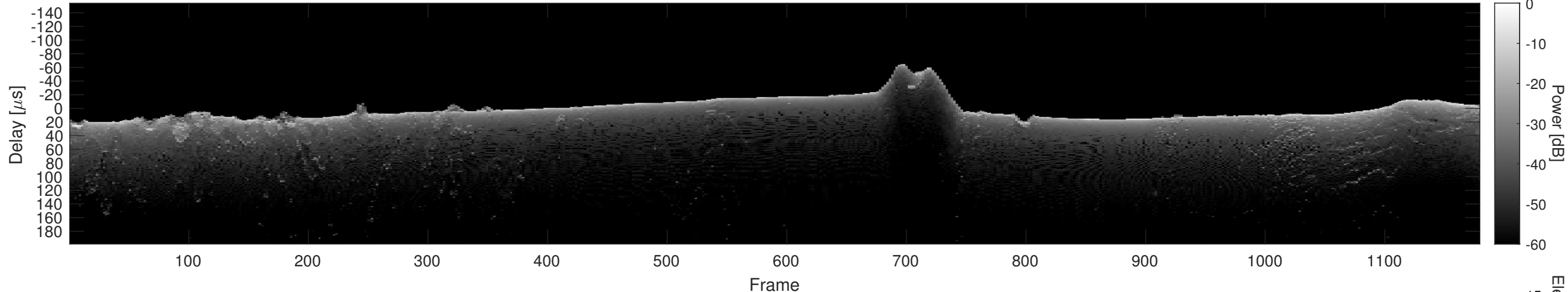
Orbit 18727, Cluttergram
