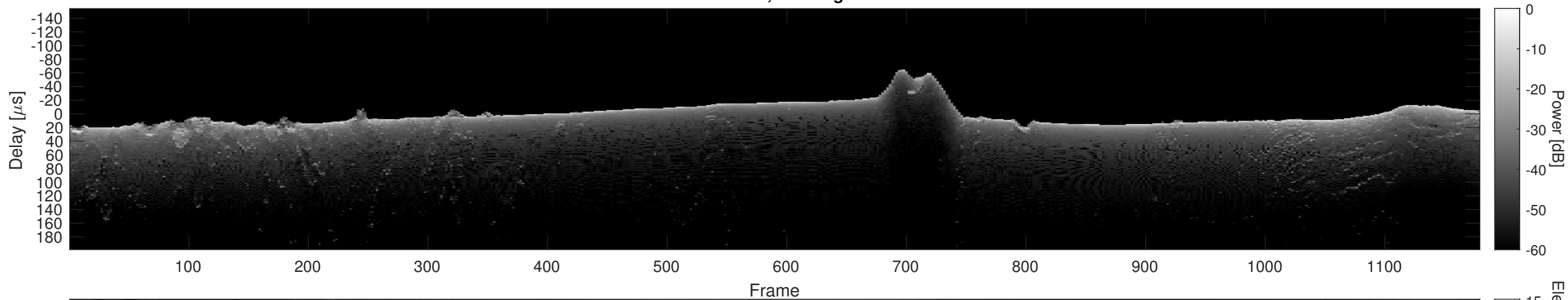
Orbit 18727, Cluttergram
