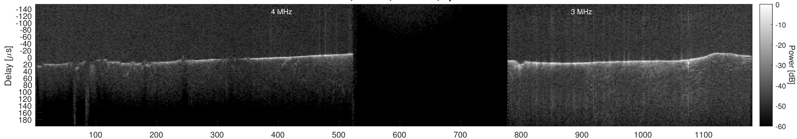
Orbit 18727, Cluttergram
