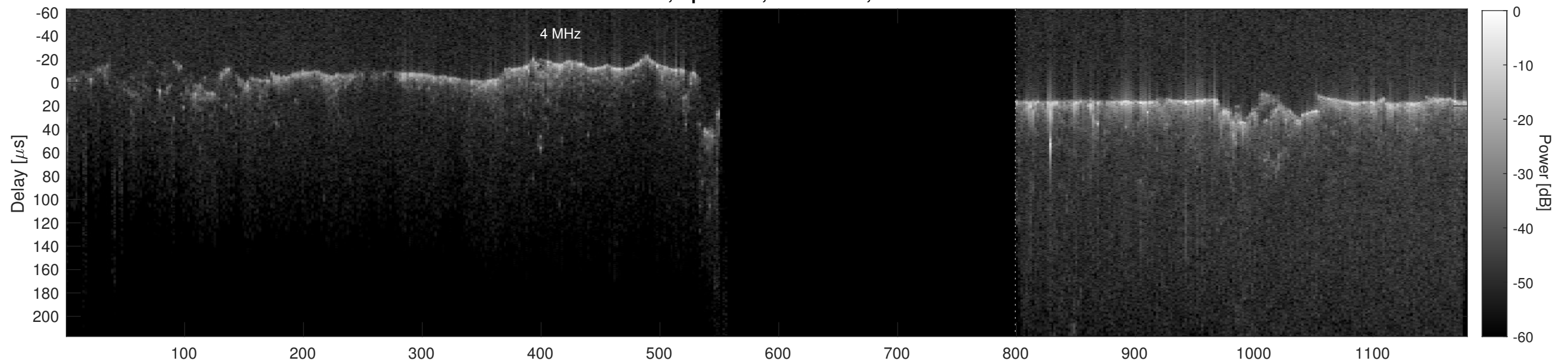
Orbit 18730, Cluttergram
