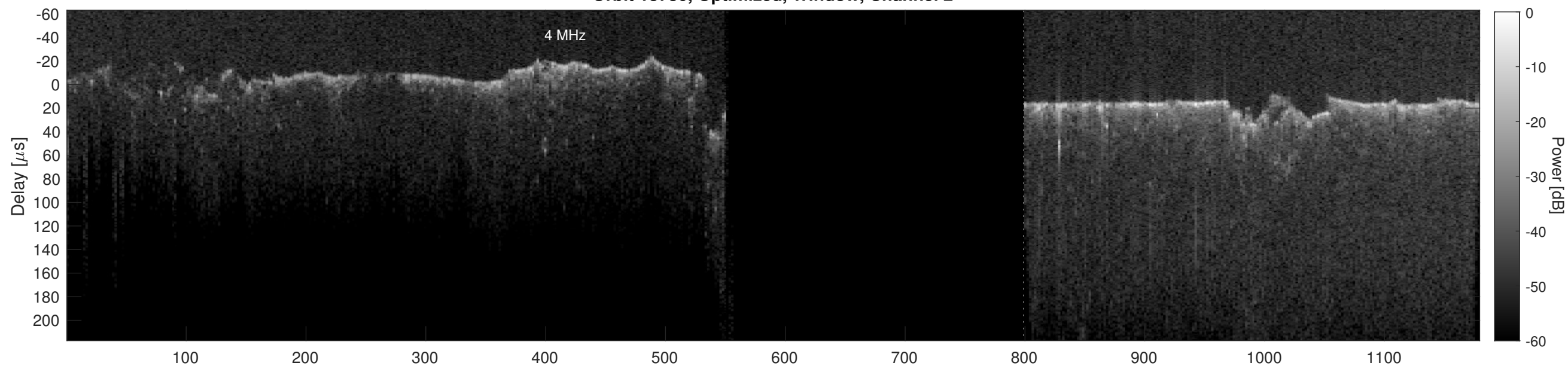
Orbit 18730, Cluttergram
