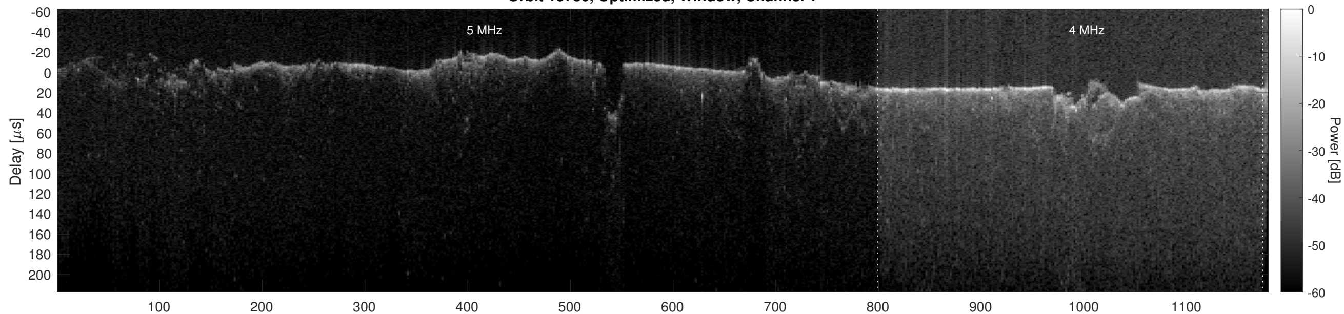
Orbit 18730, Optimized, Window, Channel 2
