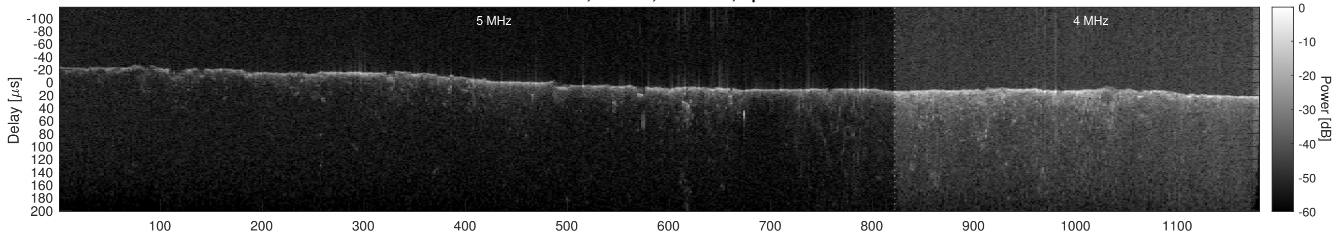
Orbit 18733, Cluttergram
