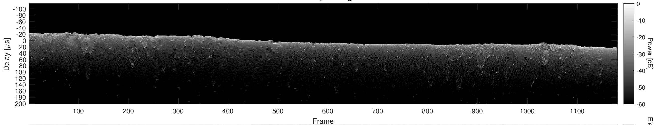
Orbit 18733, Cluttergram
