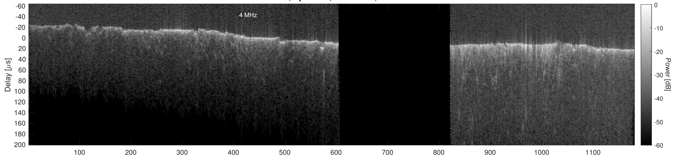
Orbit 18733, Cluttergram
