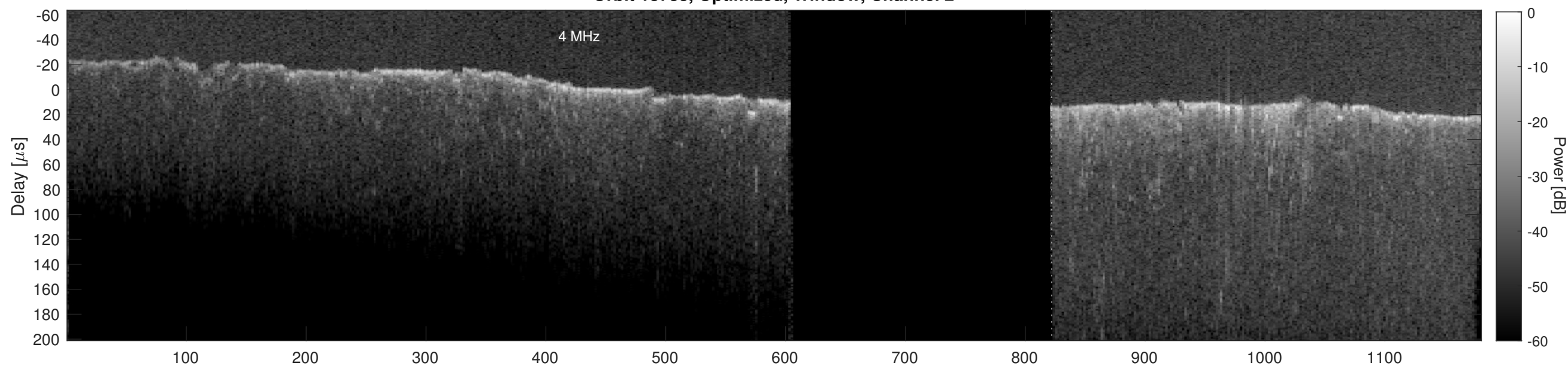
Orbit 18733, Cluttergram
