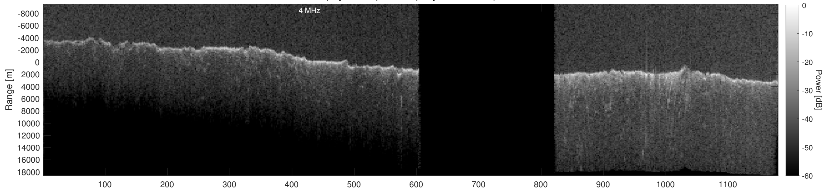
Orbit 18733, Depth-Corrected Cluttergram
