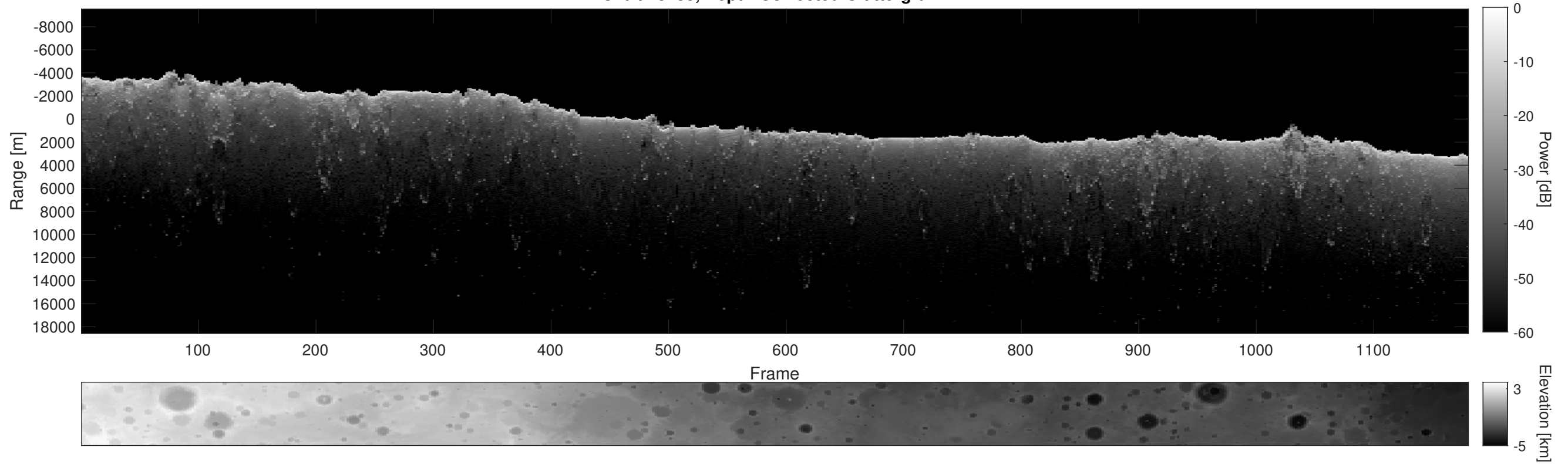
Orbit 18733, Depth-Corrected Cluttergram
