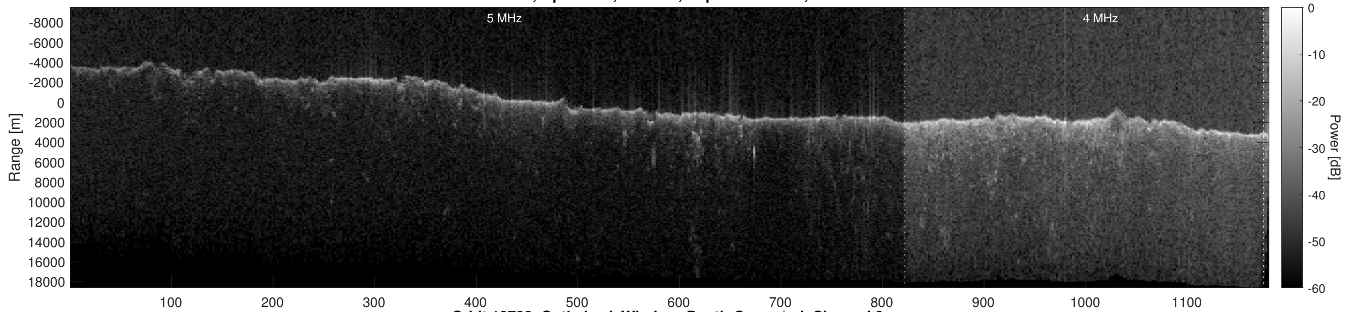
Orbit 18733, Optimized, Window, Depth-Corrected, Channel 2
