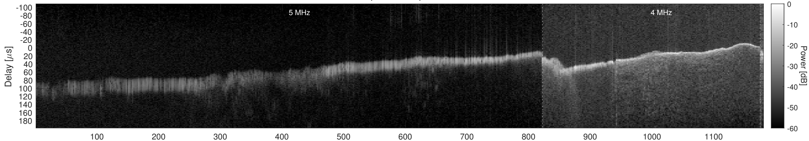
Orbit 18734, Window, Channel 1, Chapman
