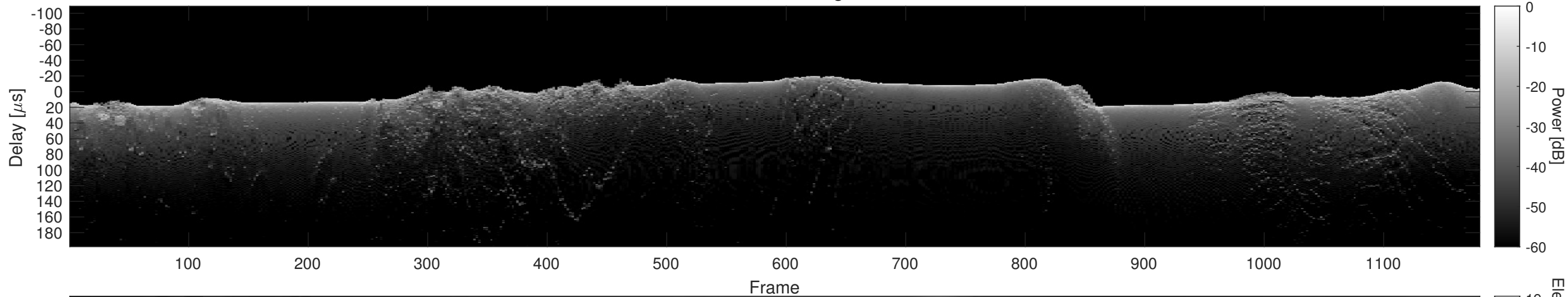
Orbit 18734, Cluttergram
