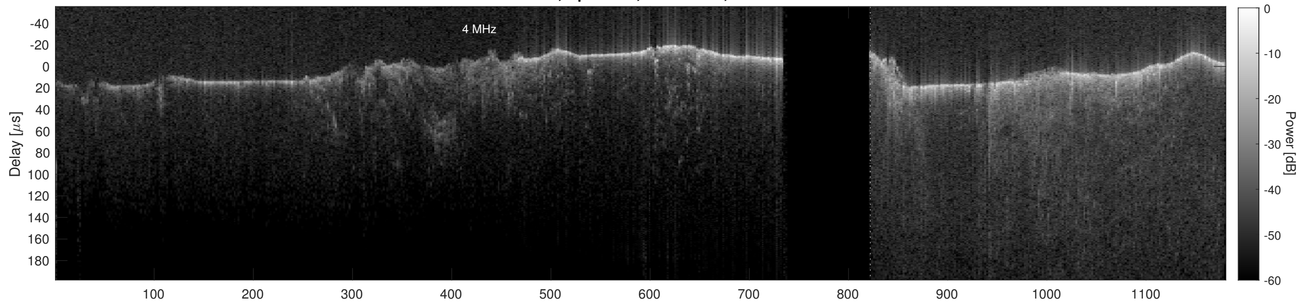
Orbit 18734, Cluttergram
