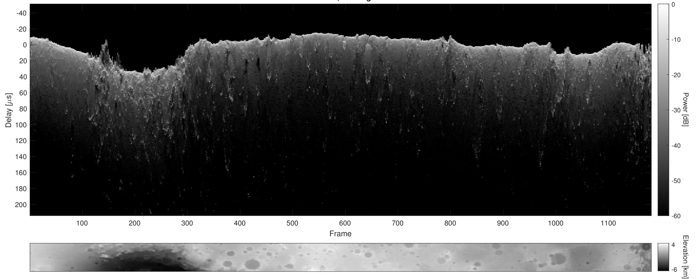
Orbit 18736, Cluttergram
