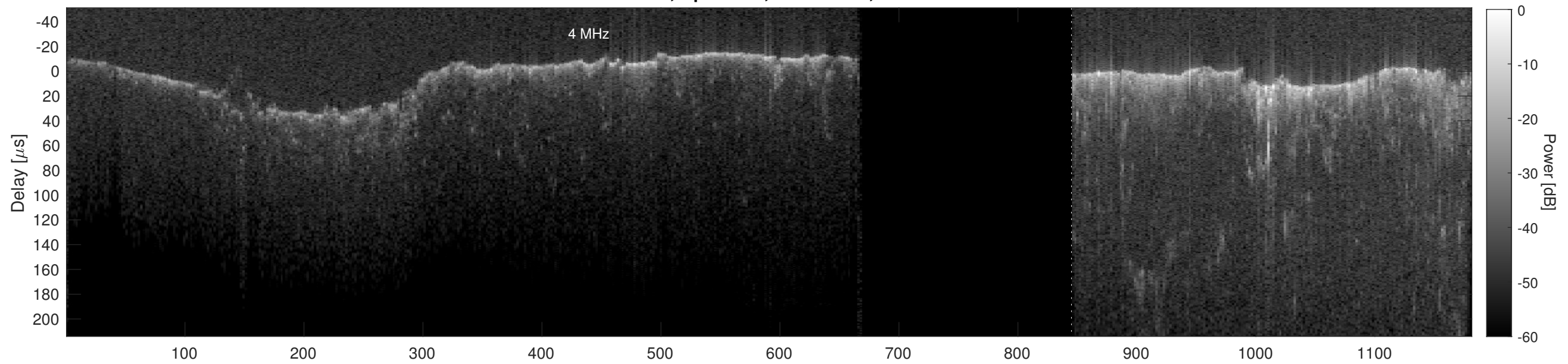
Orbit 18736, Cluttergram
