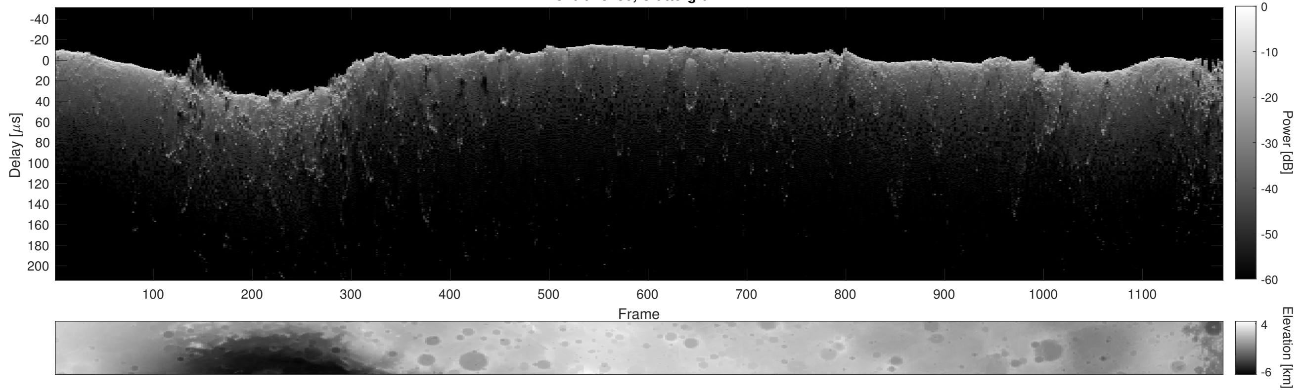
Orbit 18736, Cluttergram
