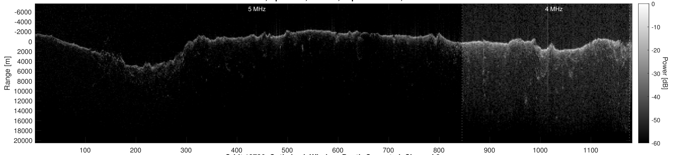
Orbit 18736, Optimized, Window, Depth-Corrected, Channel 2
