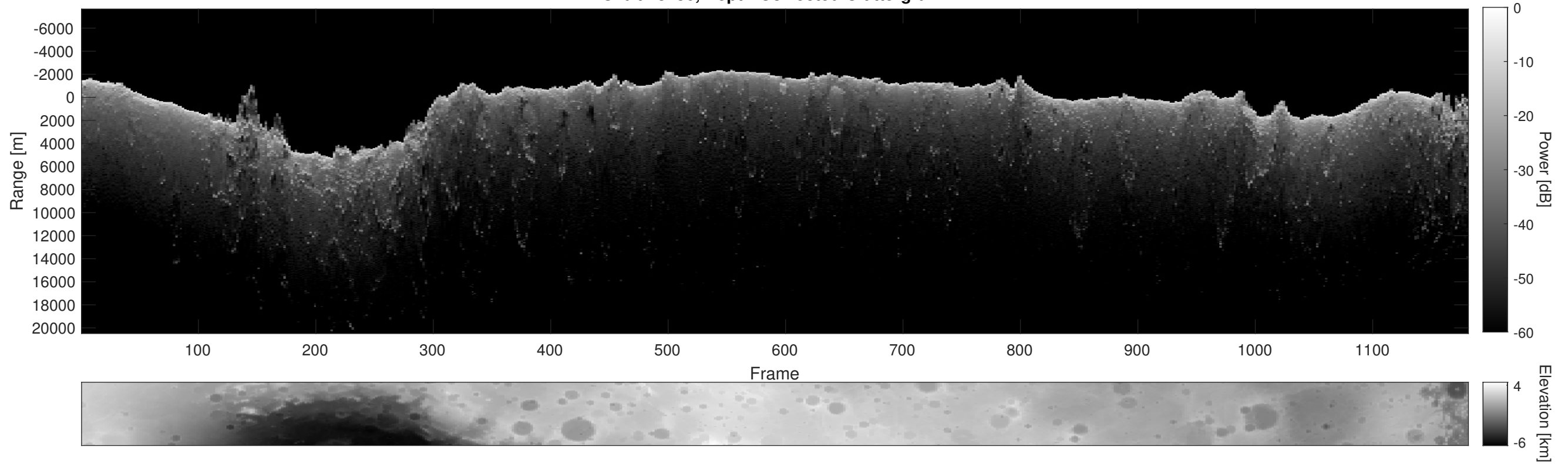
Orbit 18736, Depth-Corrected Cluttergram
