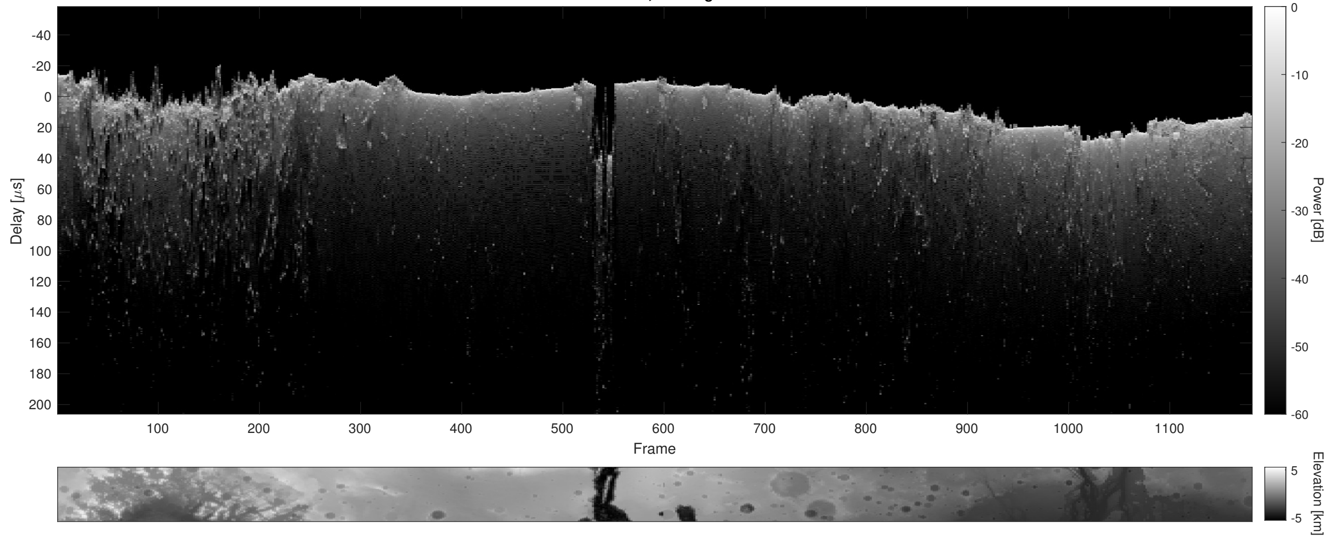
Orbit 18737, Cluttergram
