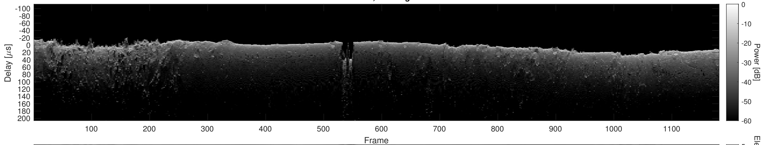
Orbit 18737, Cluttergram
