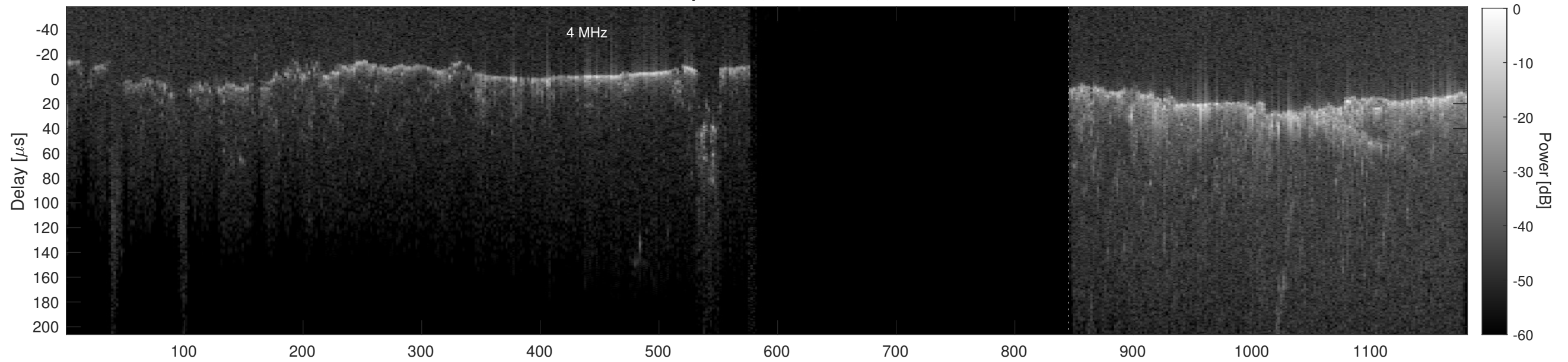
Orbit 18737, Cluttergram
