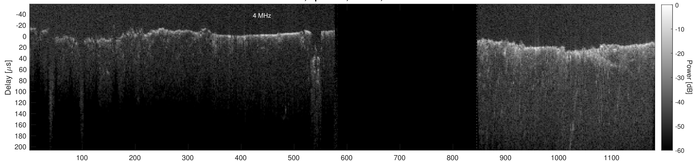
Orbit 18737, Cluttergram
