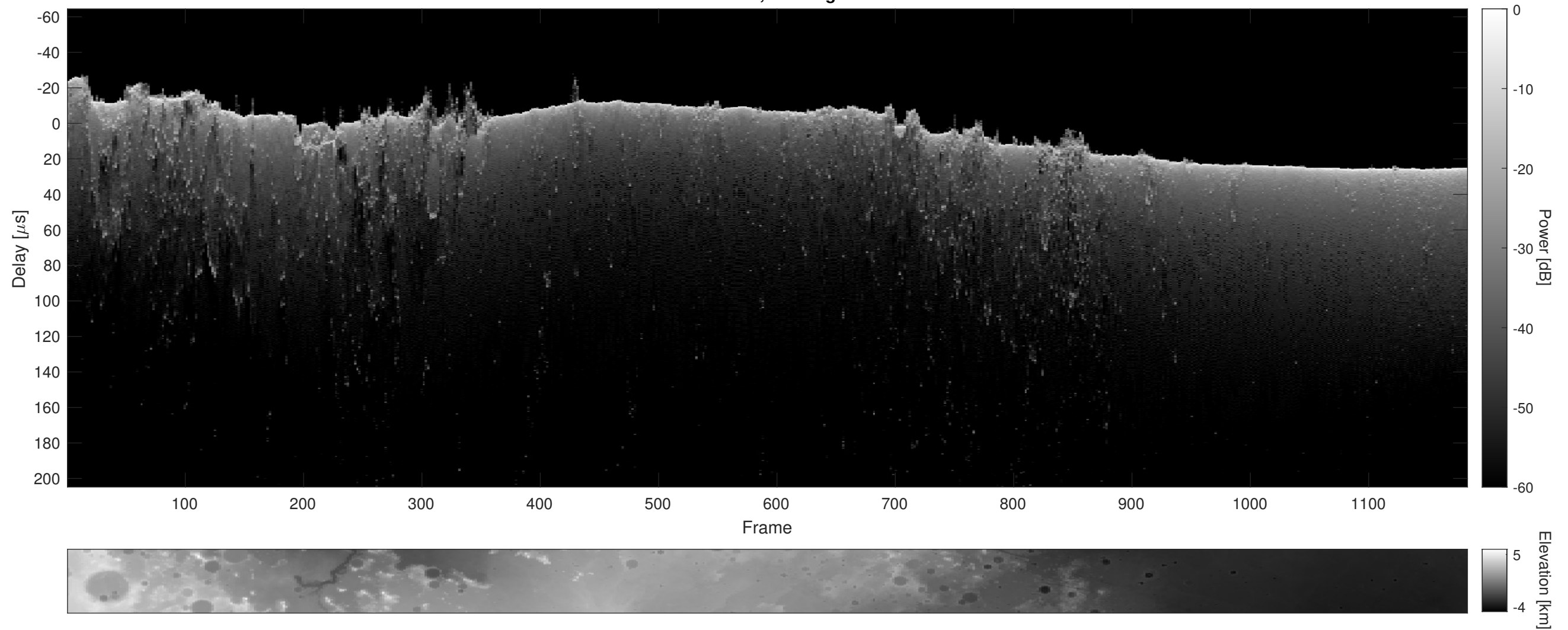
Orbit 18739, Cluttergram
