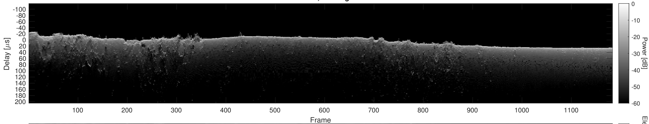
Orbit 18739, Cluttergram
