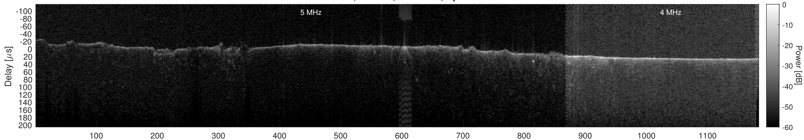
Orbit 18739, Cluttergram
