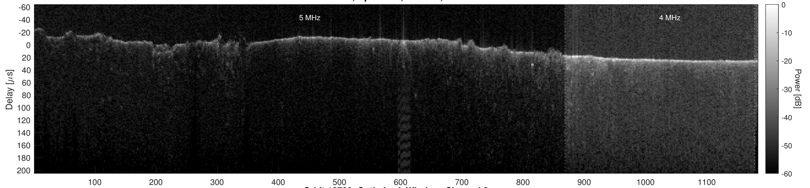
Orbit 18739, Optimized, Window, Channel 2
