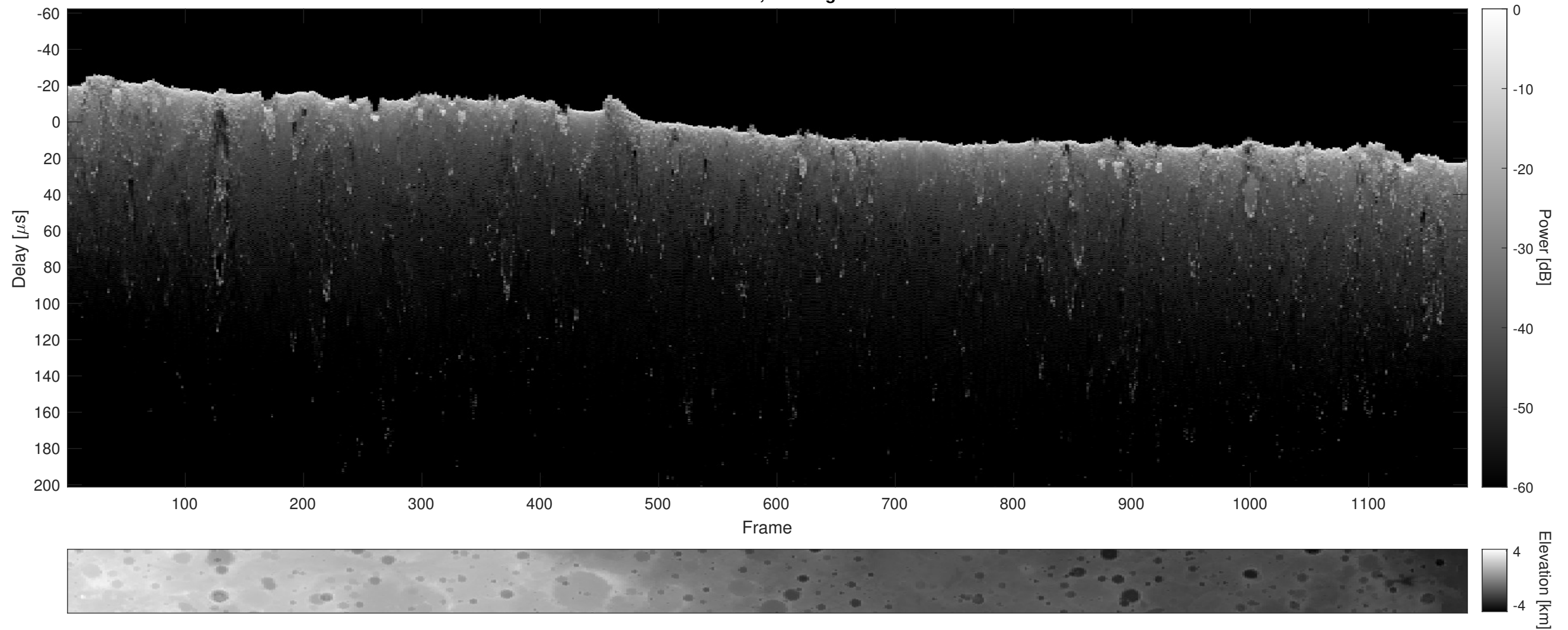
Orbit 18740, Cluttergram
