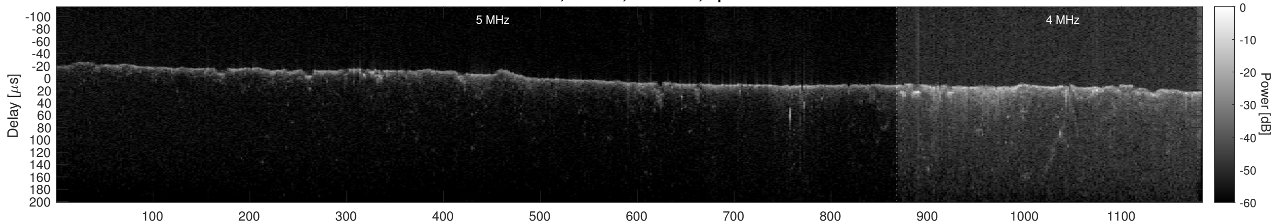
Orbit 18740, Cluttergram
