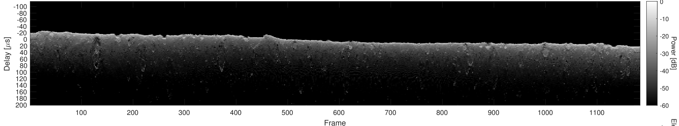
Orbit 18740, Cluttergram
