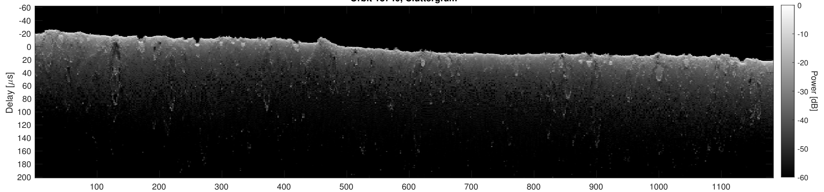
Orbit 18740, Cluttergram
