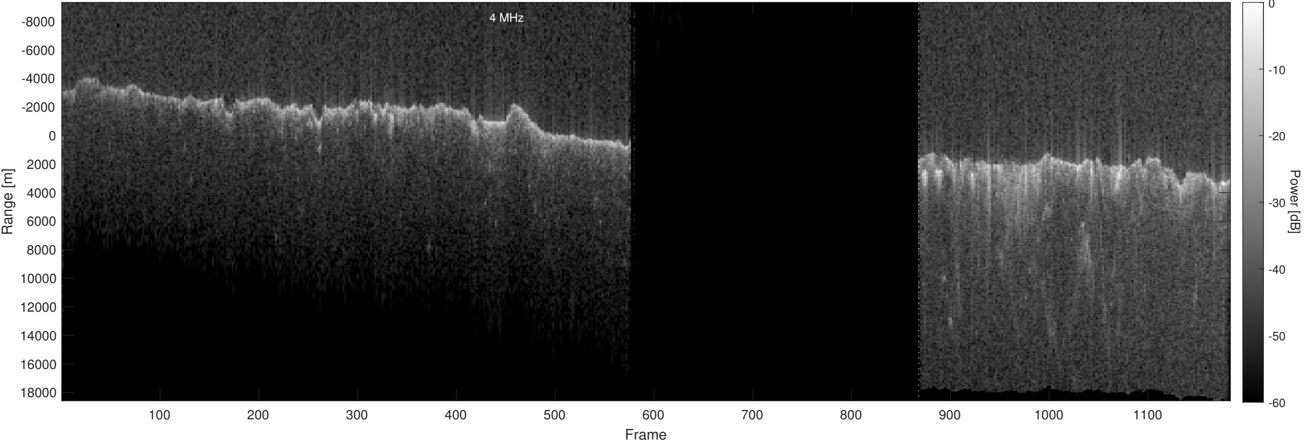
Orbit 18740, Optimized, No Window, Depth-Corrected, Channel 2
