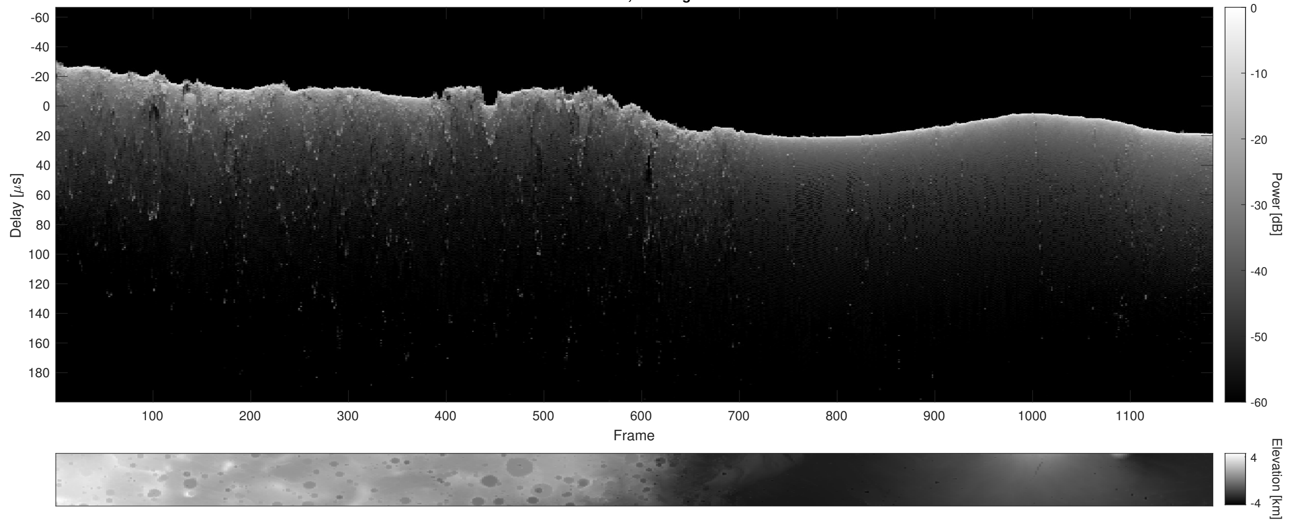
Orbit 18742, Cluttergram
