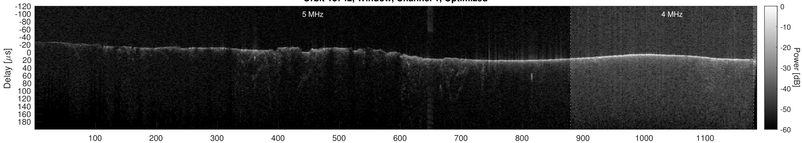
Orbit 18742, Cluttergram
