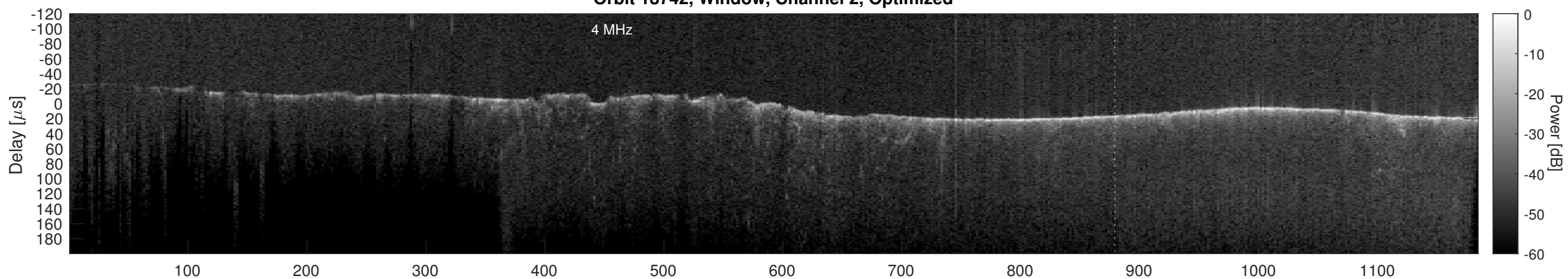
Orbit 18742, Cluttergram
