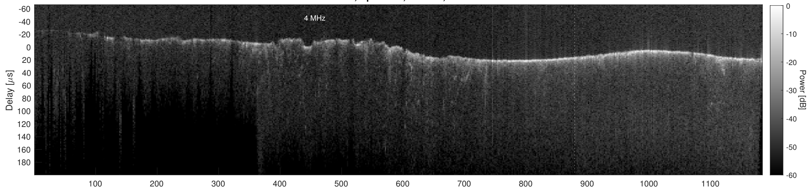
Orbit 18742, Cluttergram
