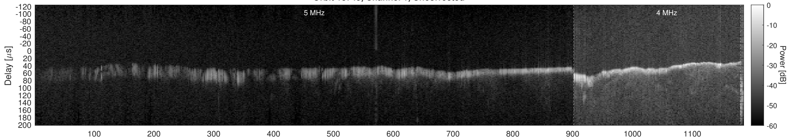
Orbit 18745, Window, Channel 1, Chapman
