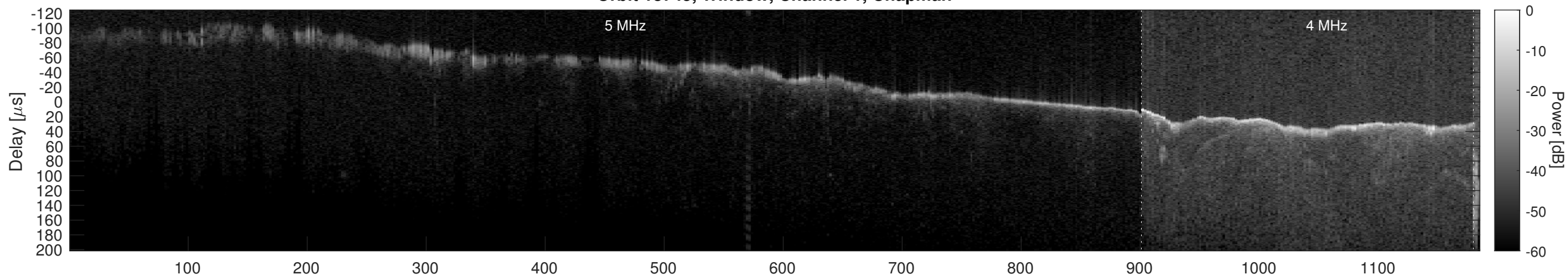
Orbit 18745, Window, Channel 1, Optimized
