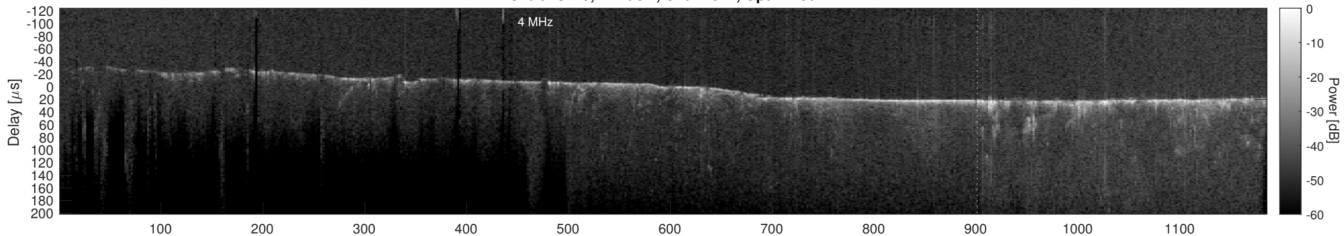
Orbit 18745, Cluttergram
