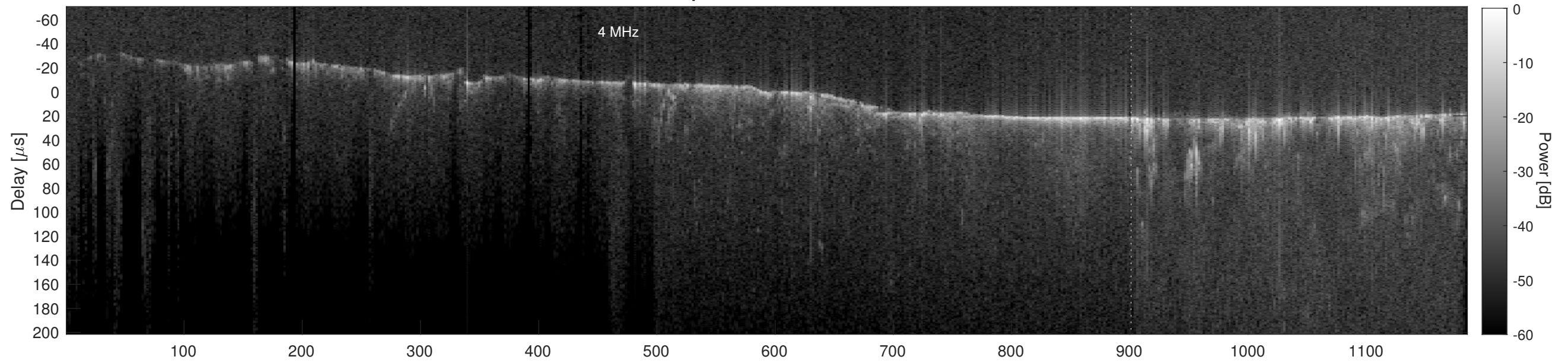
Orbit 18745, Cluttergram
