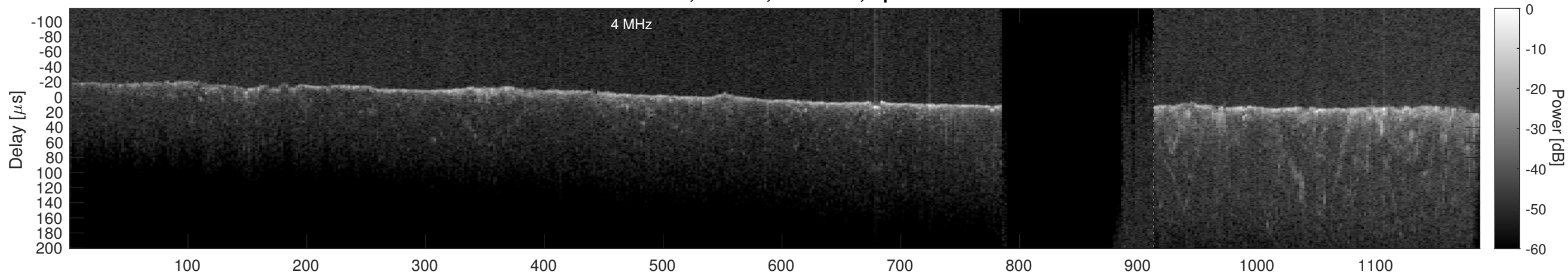
Orbit 18747, Cluttergram
