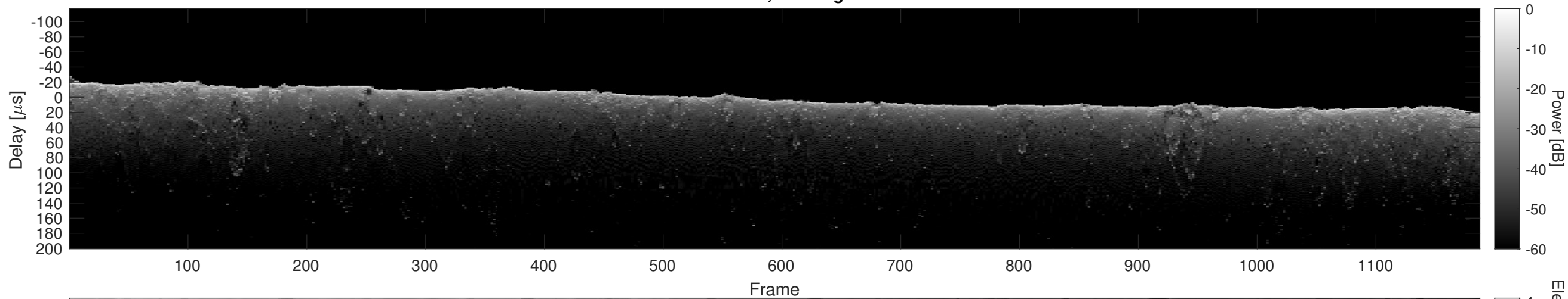
Orbit 18747, Cluttergram
