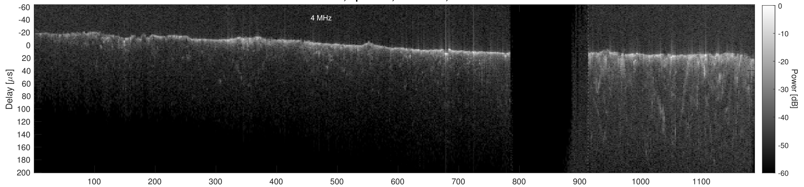
Orbit 18747, Cluttergram
