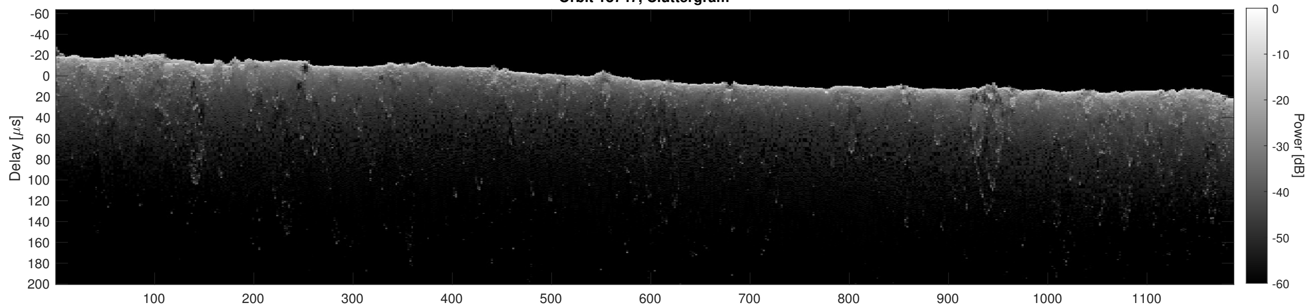
Orbit 18747, Cluttergram
