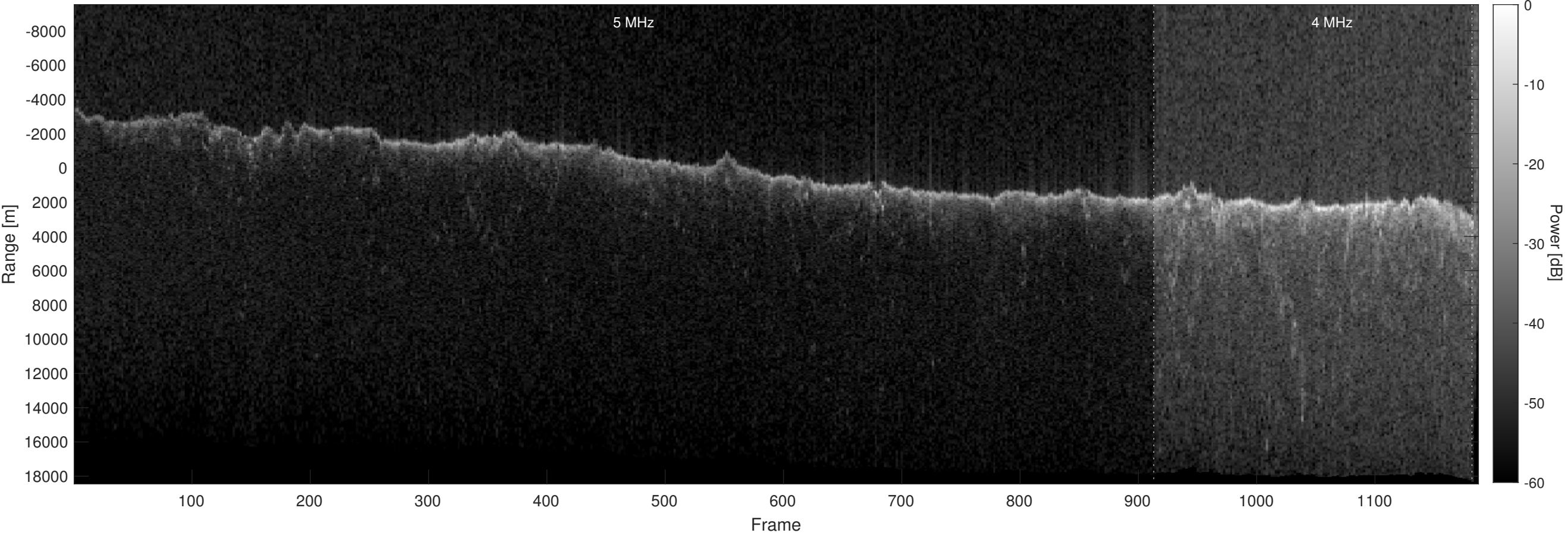
Orbit 18747, Optimized, Window, Depth-Corrected, Channel 2
