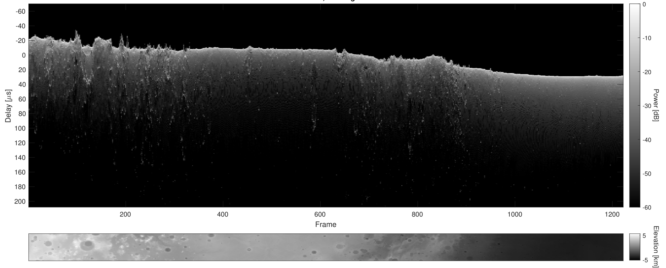
Orbit 18753, Cluttergram
