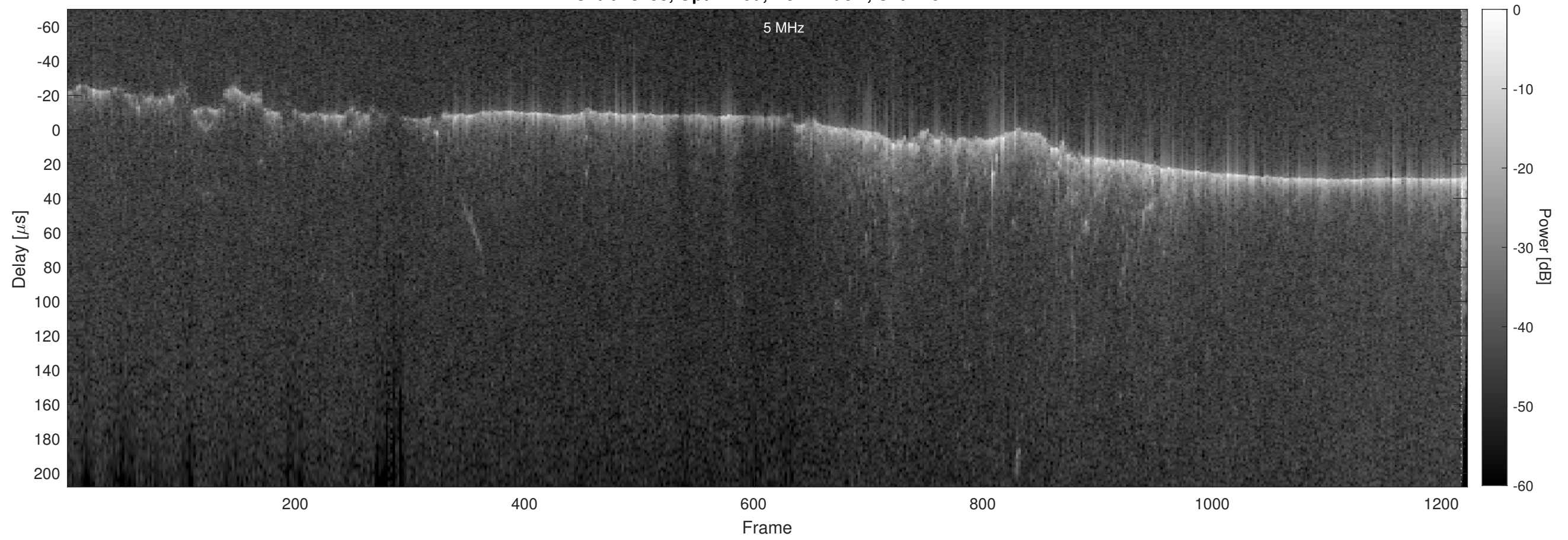
Orbit 18753, Optimized, No Window, Channel 2
