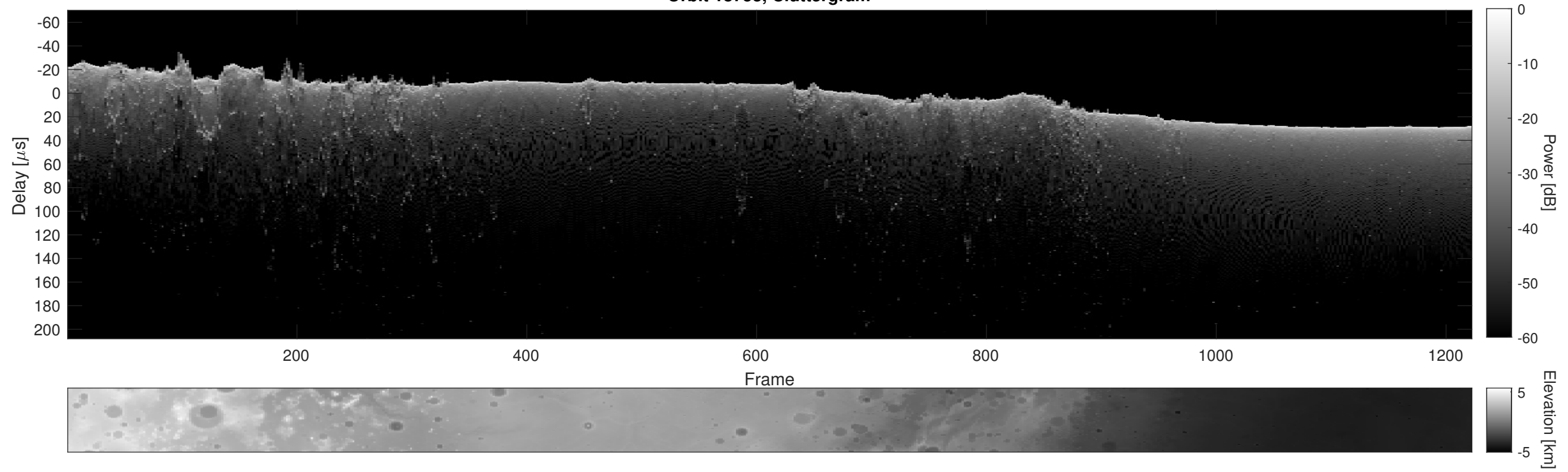
Orbit 18753, Cluttergram
