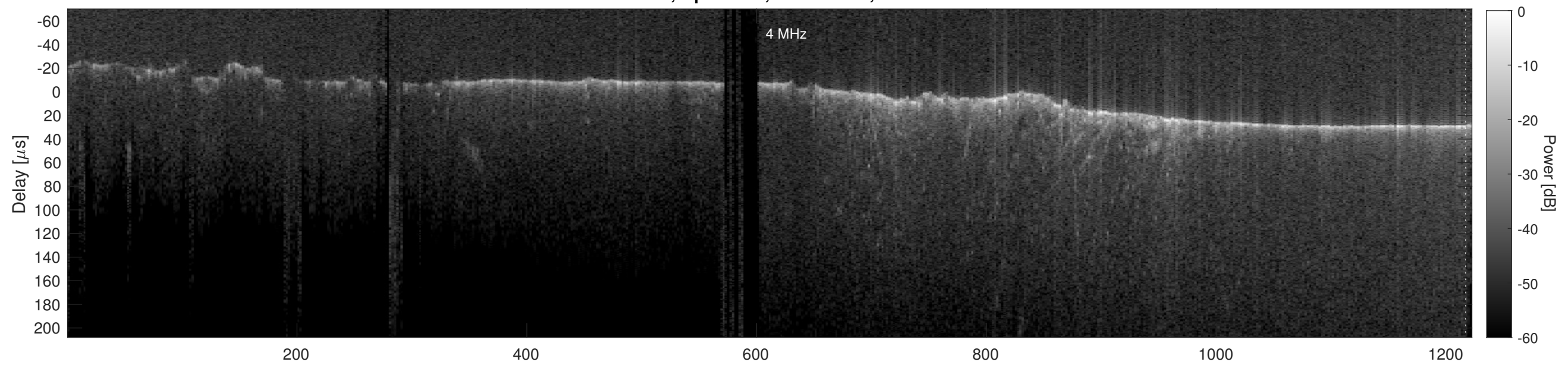
Orbit 18753, Cluttergram
