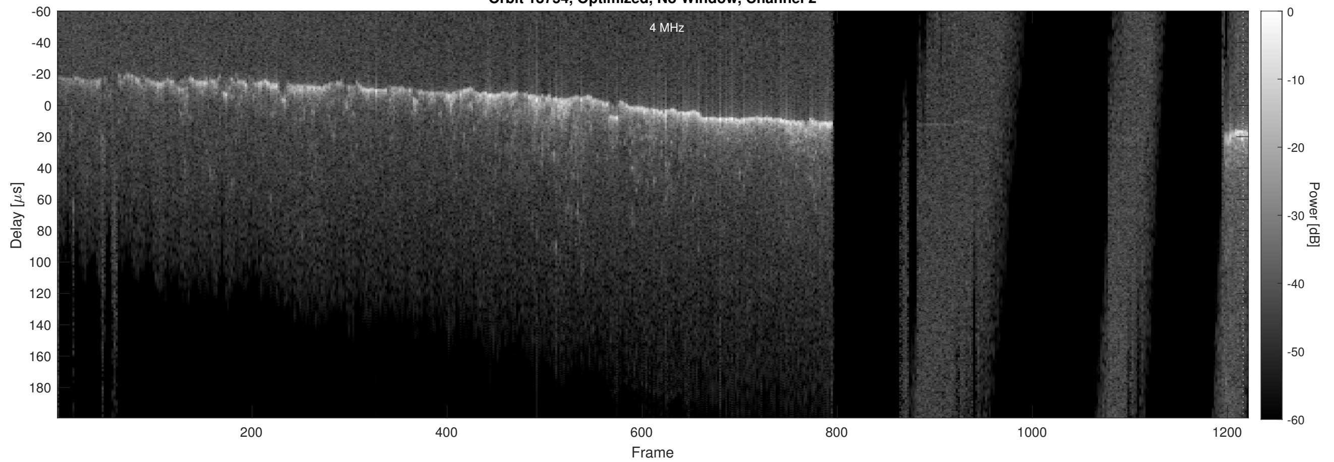
Orbit 18754, Optimized, No Window, Channel 2
