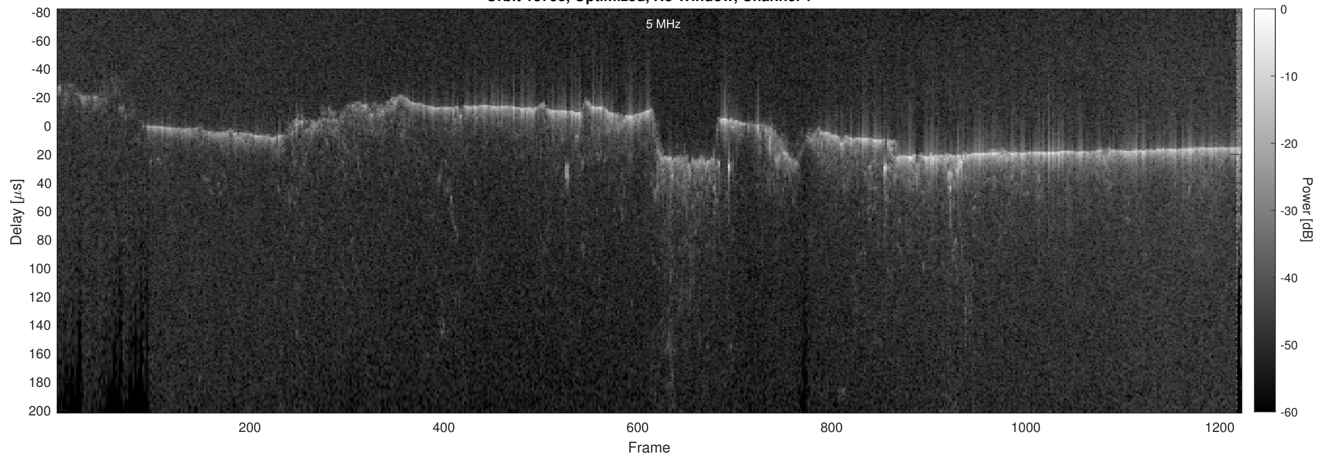
Orbit 18758, Optimized, No Window, Channel 2
