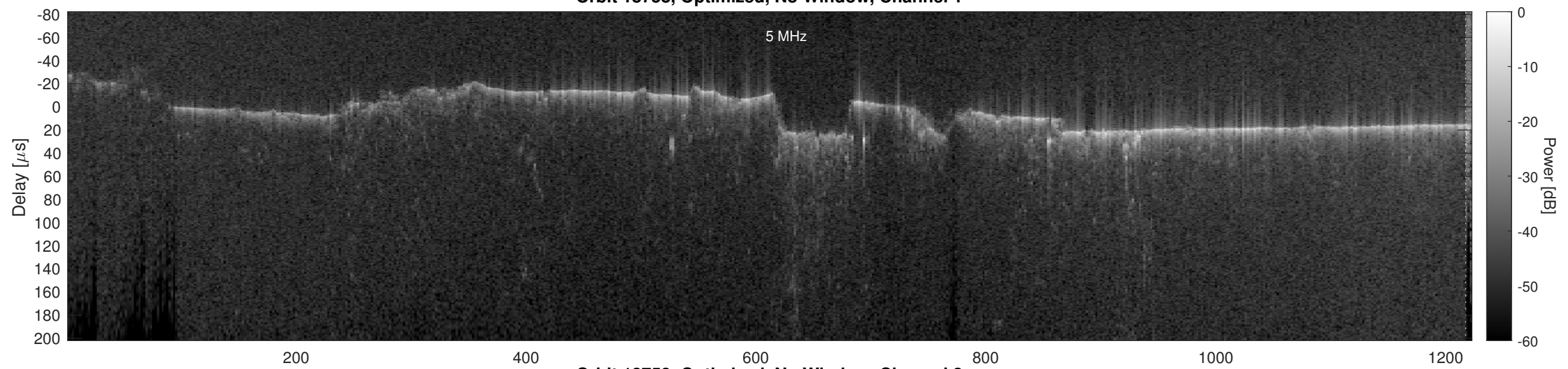
Orbit 18758, Optimized, No Window, Channel 2
